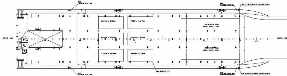
PASSENGER CAR & 15TON MIXER TRUCK LOADING PLAN
