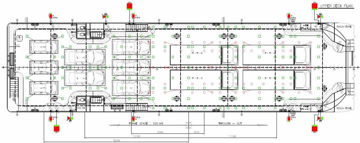
D. 5 TON CARGO TRUCK LOADING CONDITION
